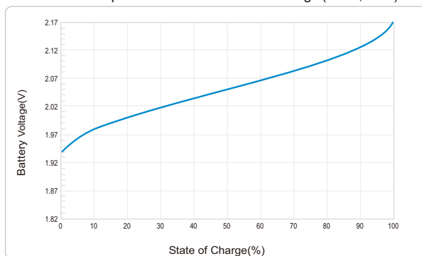
Relationship of OCV and State Of Charge(25°C,77°F)
