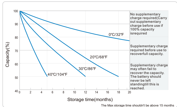
Self-discharge Characteristic
