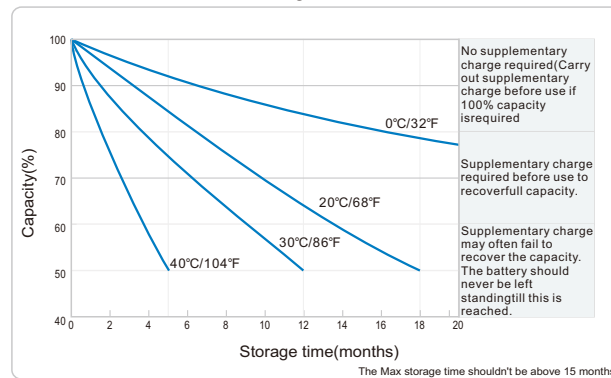
Self-discharge Characteristic
